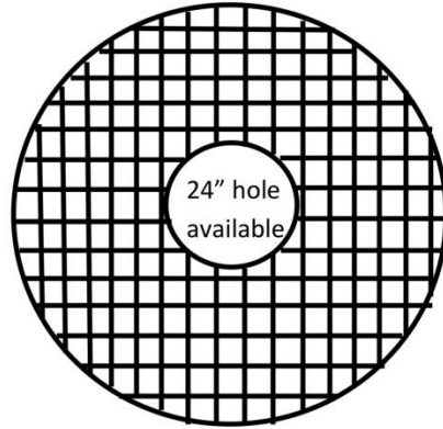
1/2" Rebar 6" apart, 6"x6" squares
